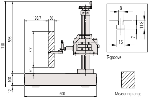
Dimensions of SJ-500 with manual column stand Unit: mm
