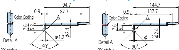
2X stylus 12AAC740 (2µm)* ( ): Tip radius 12AAB413 (5µm)** *Tip angle: 60° 12AAB425 (10µm)** **Tip angle: 90° 3X stylus 12AAC741 (2µm)* ( ): Tip radius 12AAB414 (5µm)** *Tip angle: 60° 12AAB426 (10µm)** **Tip angle: 90°
