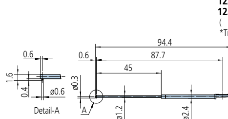
2X stylus 12AAC740 (2µm)* ( ): Tip radius 12AAB413 (5µm)** *Tip angle: 60° 12AAB425 (10µm)** **Tip angle: 90° 3X stylus 12AAC741 (2µm)* ( ): Tip radius 12AAB414 (5µm)** *Tip angle: 60° 12AAB426 (10µm)** **Tip angle: 90°
