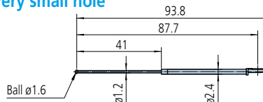
12AAE884 (0.8mm) ( ): Tip radius
