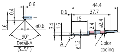
12AAC732 (2µm)* 12AAB404 (5µm)** 12AAB416 (10µm)** ( ): Tip radius *Tip angle: 60° **Tip angle: 90°
