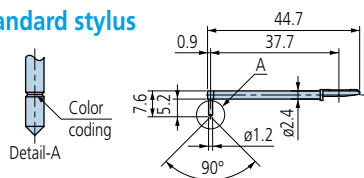
12AAE882 (1µm)* 12AAE924 (1µm)** 12AAC731 (2µm)* 12AAB403 (5µm)** 12AAB415 (10µm)** 12AAE883 (250µm) ( ): Tip radius *Tip angle: 60° **Tip angle: 90°
