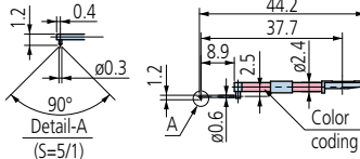
12AAC733 (2µm)* 12AAB405 (5µm)** 12AAB417 (10µm)** ( ): Tip radius *Tip angle: 60° **Tip angle: 90°
