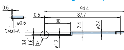
12AAE892 (2µm)* 12AAE908 (5µm)** ( ): Tip radius *Tip angle: 60° **Tip angle: 90°
