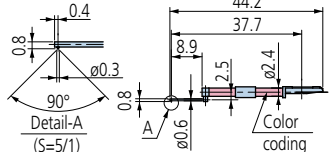
12AAC734 (2µm)* 12AAB406 (5µm)** 12AAB418 (10µm)** ( ): Tip radius *Tip angle: 60° **Tip angle: 90°
